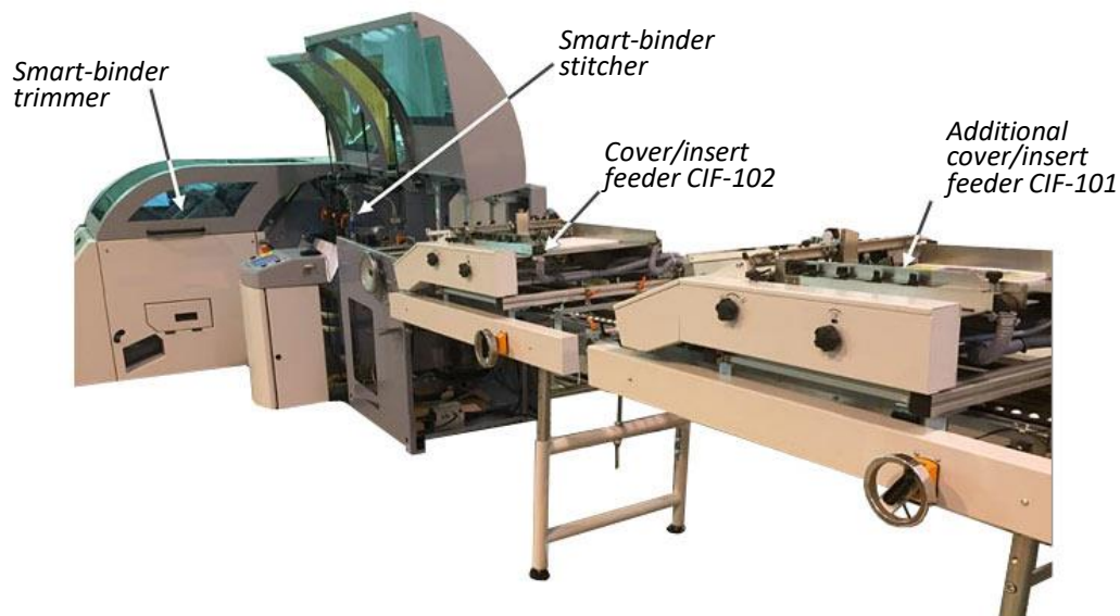
Smart-binder fitted with additional feeder CIF-101
